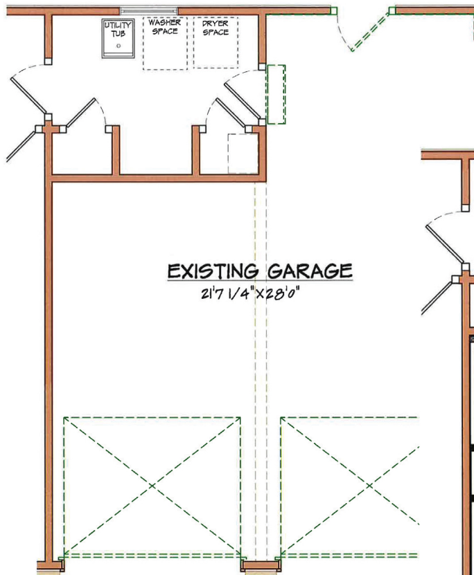
PARTIAL DEMOLITION PLAN Scale: 1/4" = 1'-0"
