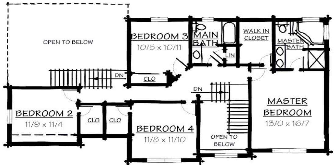
Second Floor Layout
