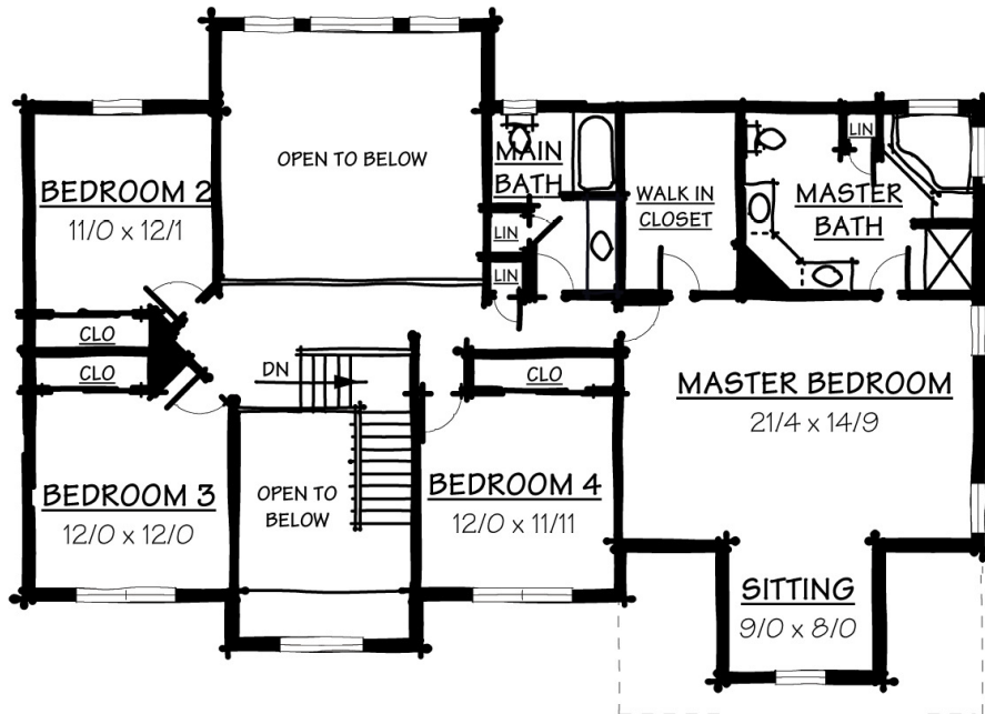
Second Floor Layout
