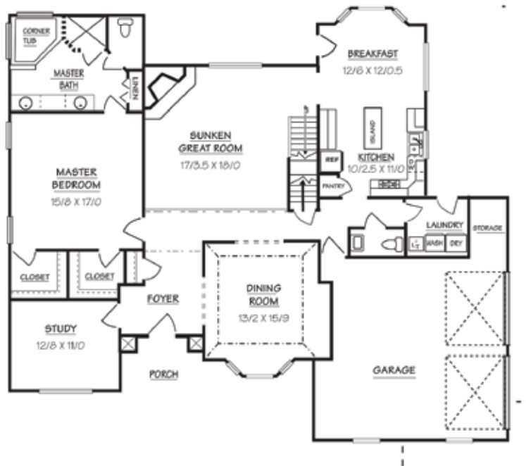
Montgomery First Floor
